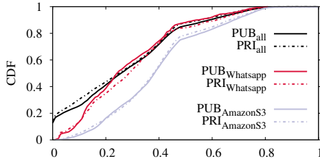
(b) Upload CDFs for flows carrying \geq 500 kB.
