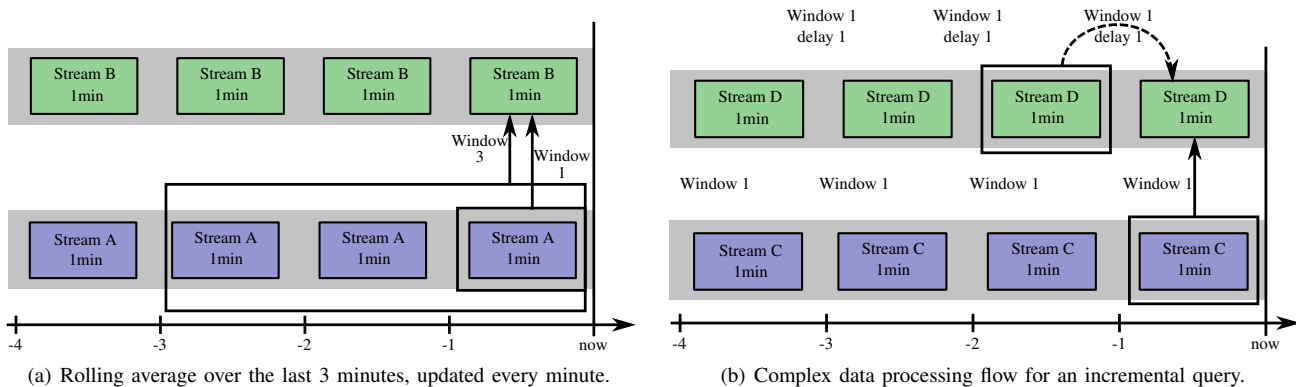
Fig. 2. Data flow of two example incremental jobs; the windows of the current task are marked in black.
